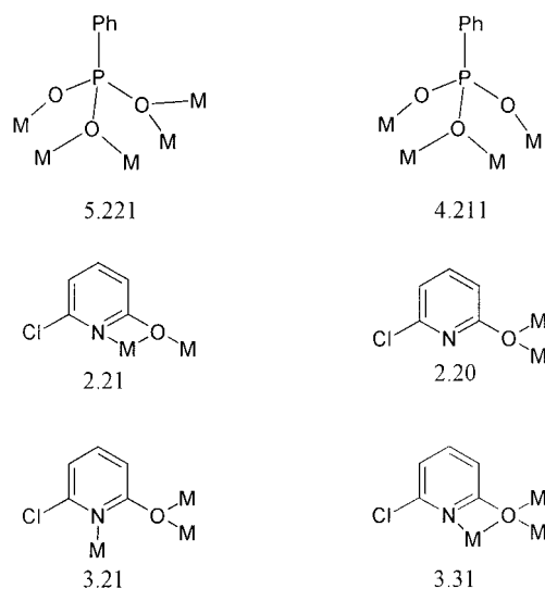
Scheme 1. The bonding modes displayed by phosphonate and pyridonate ligands, with the Harris notation for each mode.
